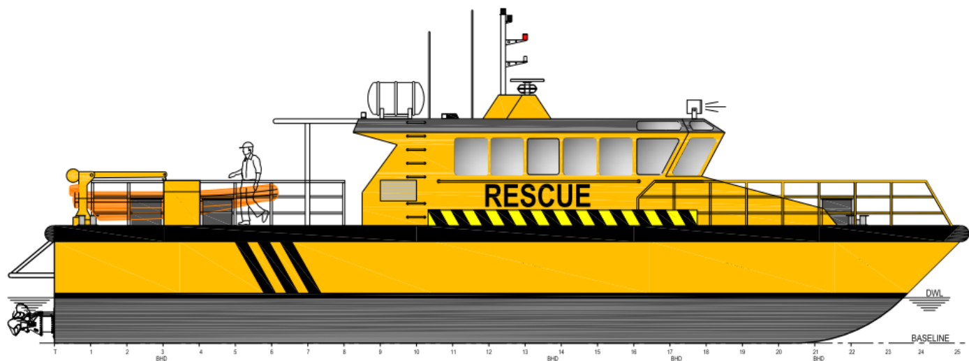
STB'D PROFILE
